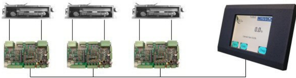
Multiple Genetix GCMs (Feeder mounted) connected to remote Color Display
